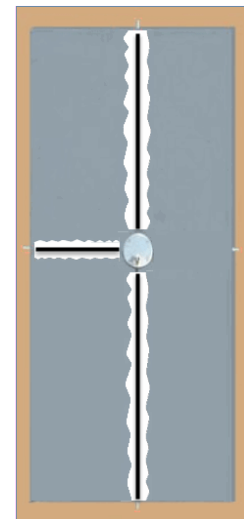
Rods Travel Within the door to project the deadbolts at three sides. The Hinge Side Bolt extends into the frame as the door closes
